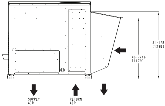
HORIZONTAL ECONOMIZER
