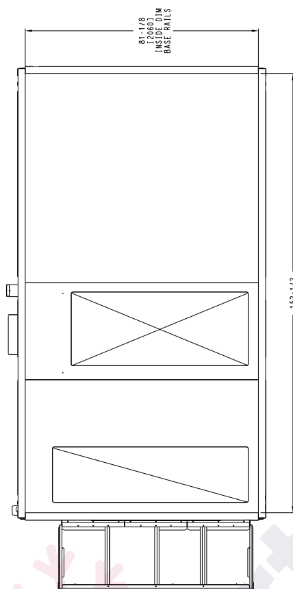
BOTTOM INSIDE BASERAIL DIMENSIONS
