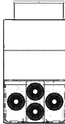
28 SIZE CONDENSER COIL TOP VIEW
